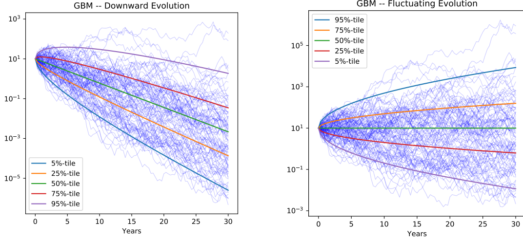
(a) Percentiles and paths of the geometric Brownian motion with drift \mu = 0 and volatility \sigma = 0.75 . Eventually, all percentiles are decreasing and converging to 0. Due to the logarithmically scaled y-axis convergence or divergence speeds might seem to be much lower than they really are; exponential behaviour appears to be only linear.
