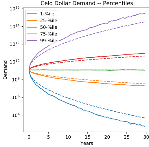
Figure 3: This figure shows empirical percentiles (sample size = 10 000) of the Celo Dollar demand processes using the parameter settings summarised in Table 1. As a reference the dashed lines show the theoretical percentiles of a geometric Ornstein-Uhlenbeck process without jumps. At each time t , 50% of the paths are above the initial value and 50% of the paths are below the initial value.
